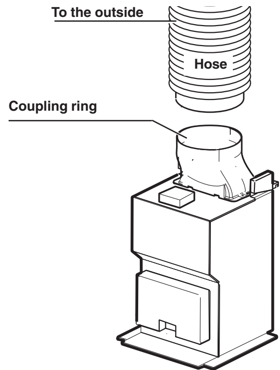
Fig. 1 - Extractor version
